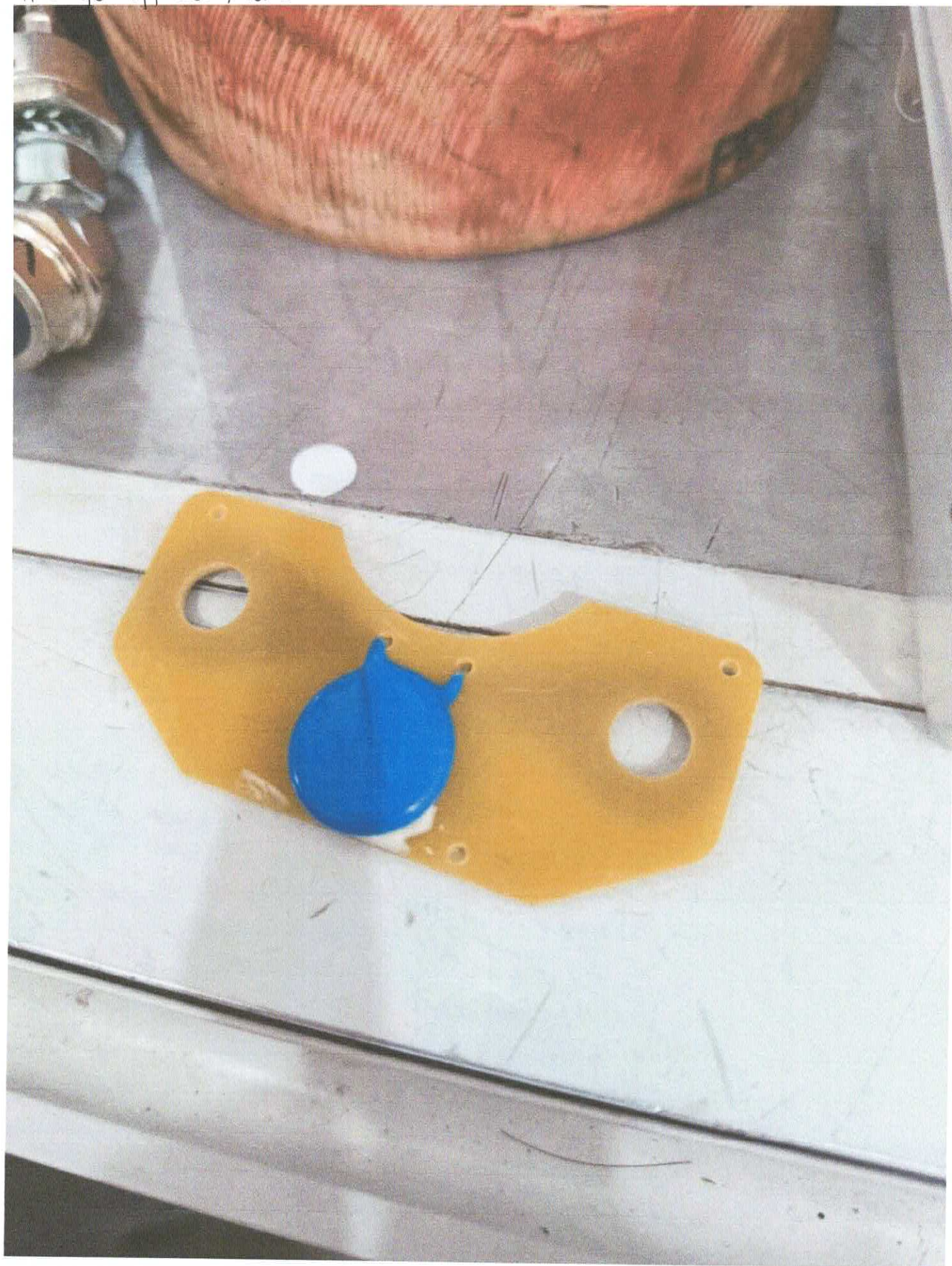
14. Surge Suppressor / Varistor
